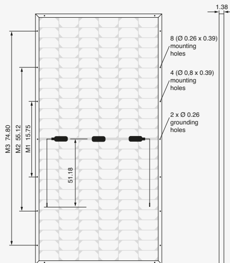
All dimensions in inch
